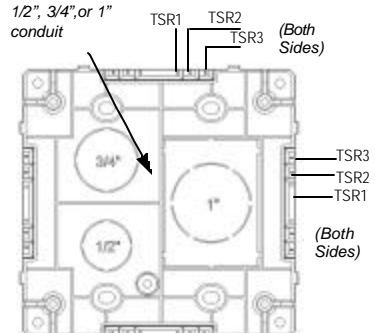
JBD - DUAL GANG
