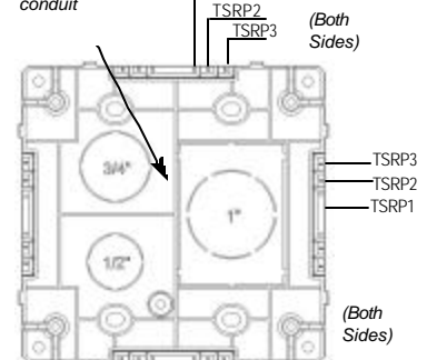
JBDP - DUAL GANG
