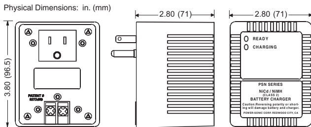
Tolerances are +/- 0.04 in. (+/- 1mm) and +/- 0.08 in. (+/- 2mm) for height dimensions.
