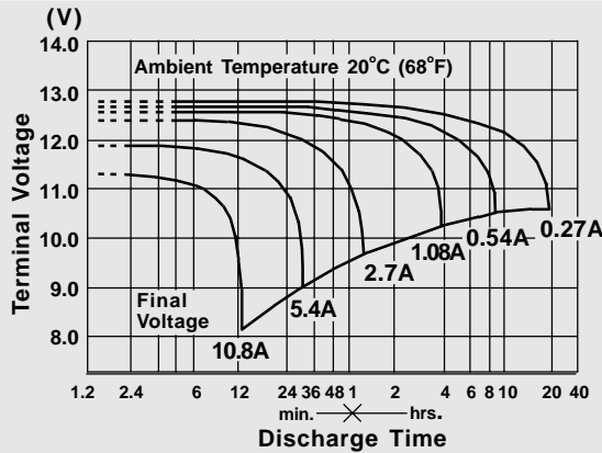
Discharge Characteristics
